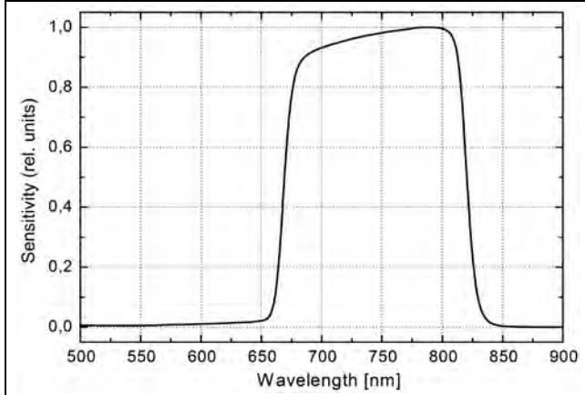
Normalized Spectral Response (preliminary)
