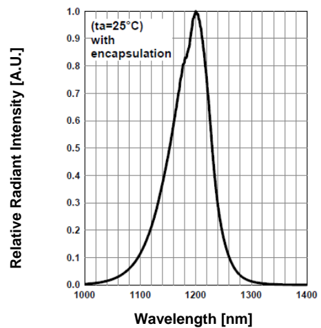
Radiation Characteristics
