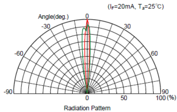
Radiation Pattern
